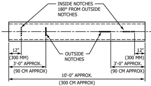
FIG. S1.1 Eddy-Current Test Standard
