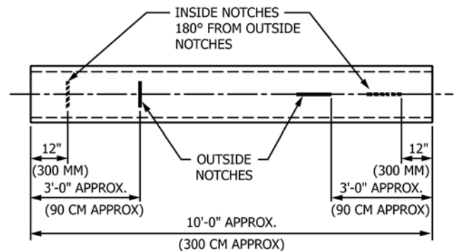
FIG. S1.1 Eddy-Current Test Standard
